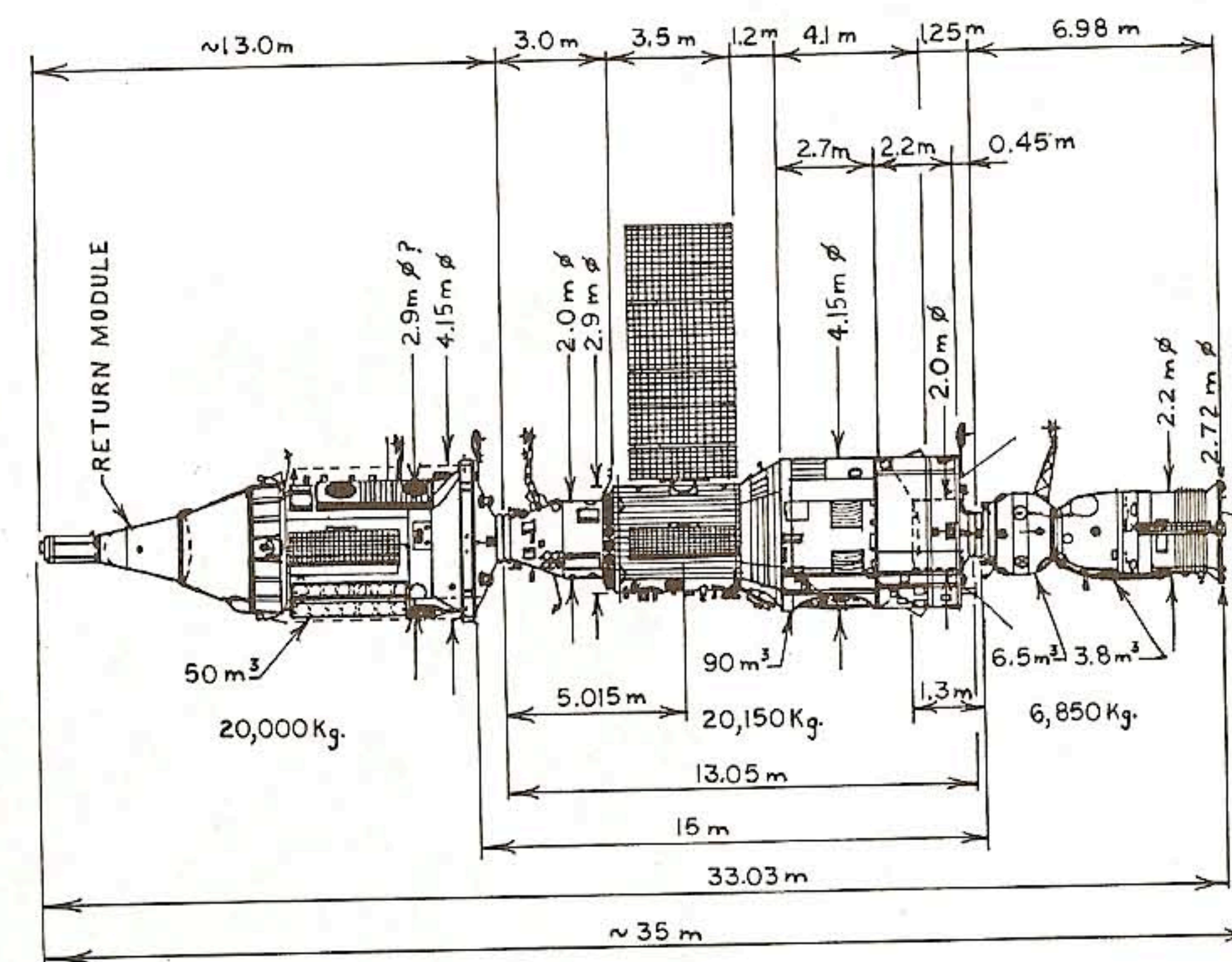
Figure 3-2. Salyut 7.
