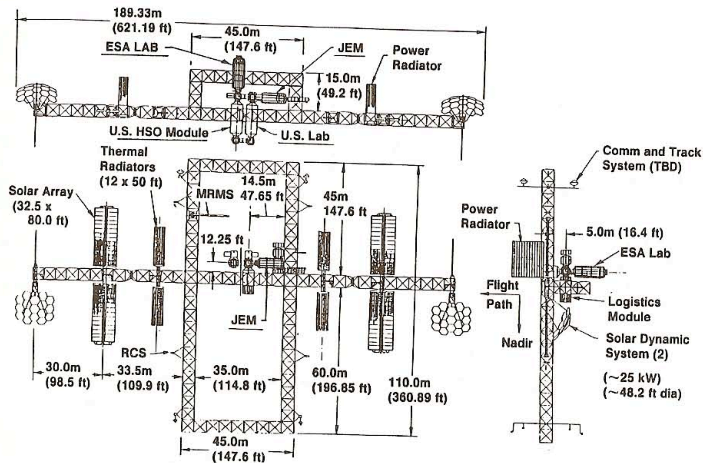
Figure 3-12. Dual Keel space station configuration.
