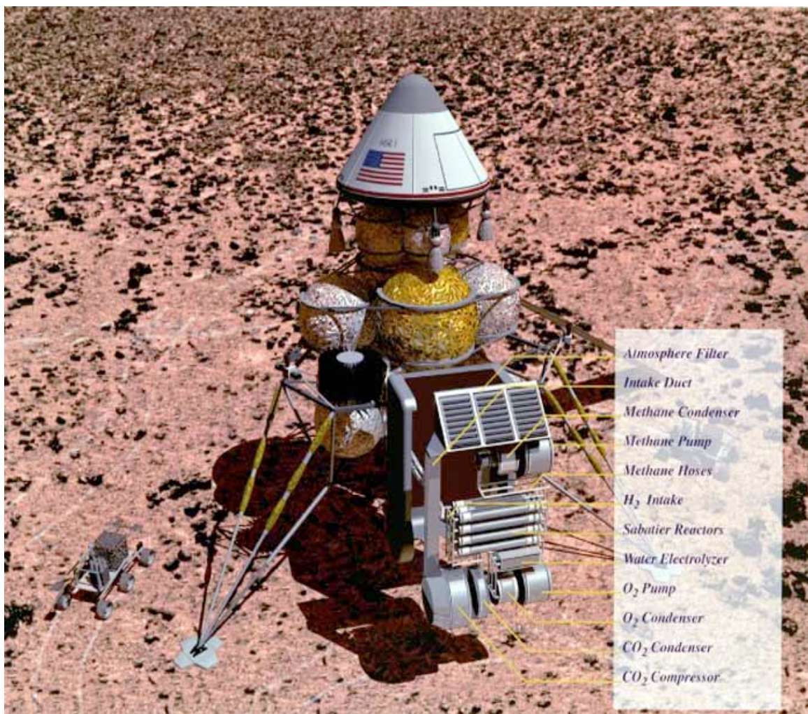
FIGURE 16. Generic conceptual model of a Mars Sample Return Ascent Vehicle, that would generate its own ISRU fuel and carry the payload of .5 kg of Mars samples in the conical capsule on top. Courtesy of NASA.
